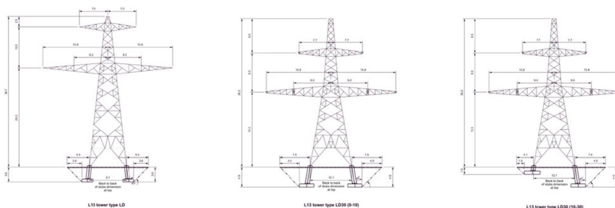
Image 5.15 Low height pylon ( document reference 2.6.2 )[APP-042]
