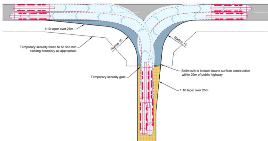
Image 5.21 Image 5.24 Illustrative bellmouth – mobile crane swept path
