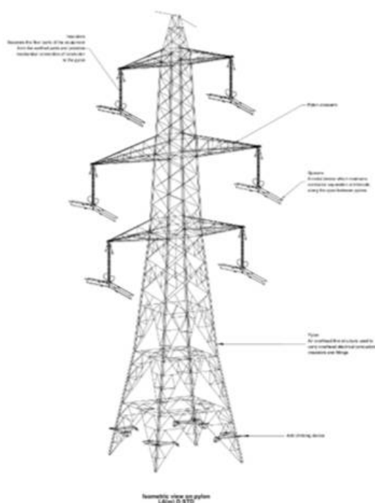
Image 5.11 Example of a 400 kV double circuit lattice pylon ( document reference 2.6.2APP-042 )
